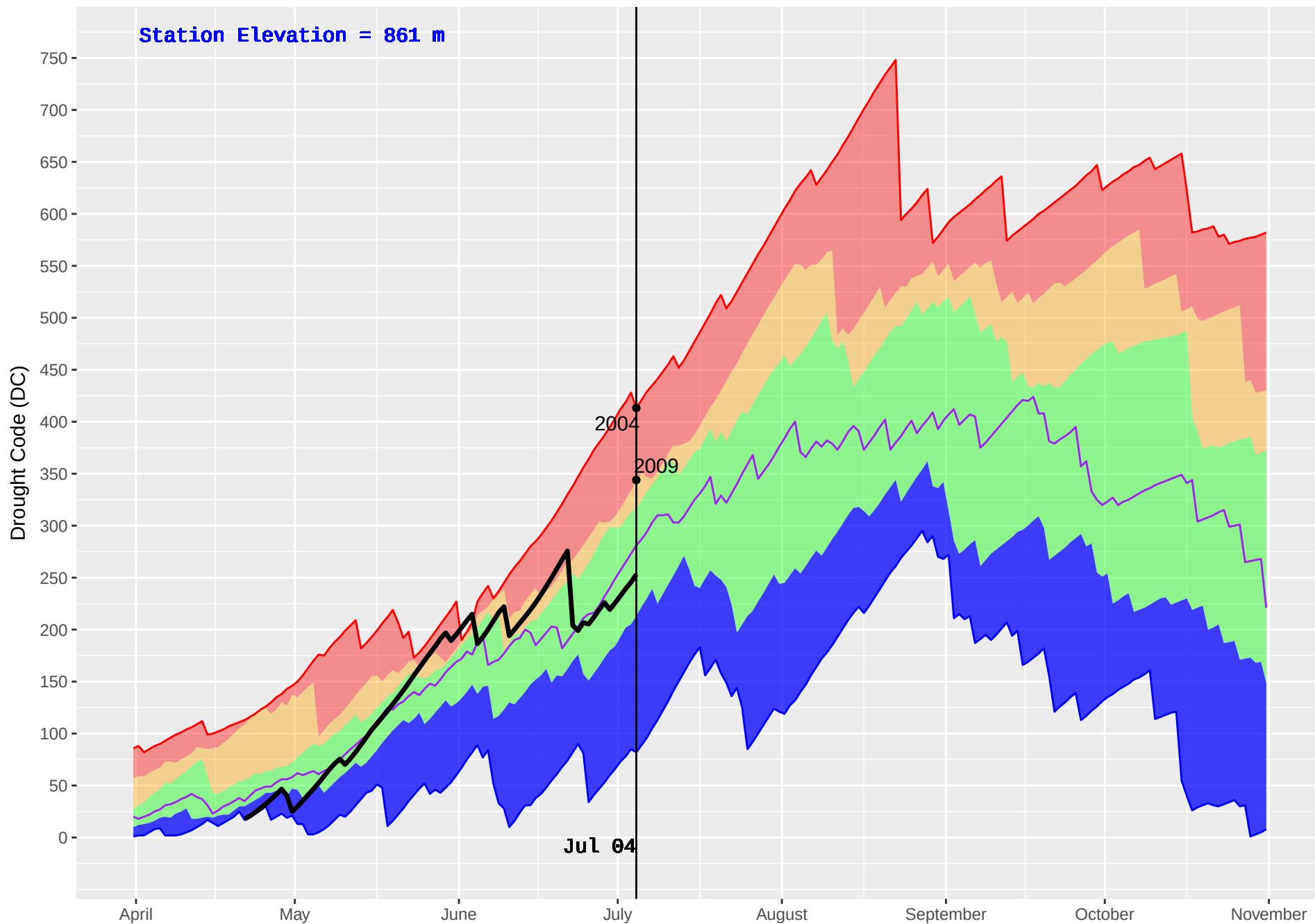
BLAEBERRY (866) : Historical (2004–2016) and Current (2018) Noon Drought Code (DC)
