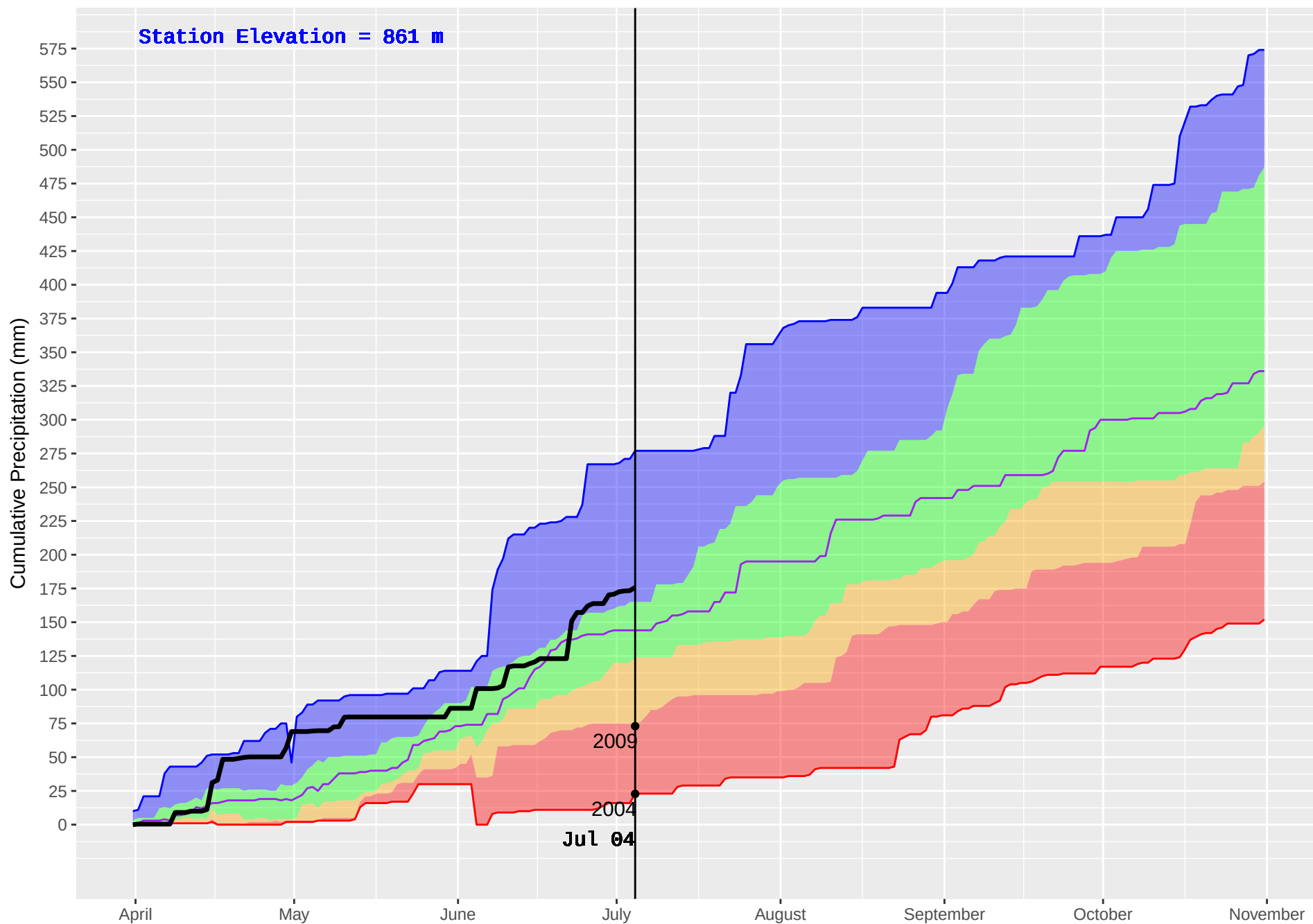
BLAEBERRY (866) : Historical (2004–2016) and Current (2018) Noon Cumulative Precipitation
